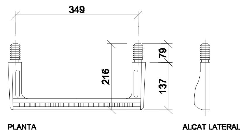
DETALL PATE
